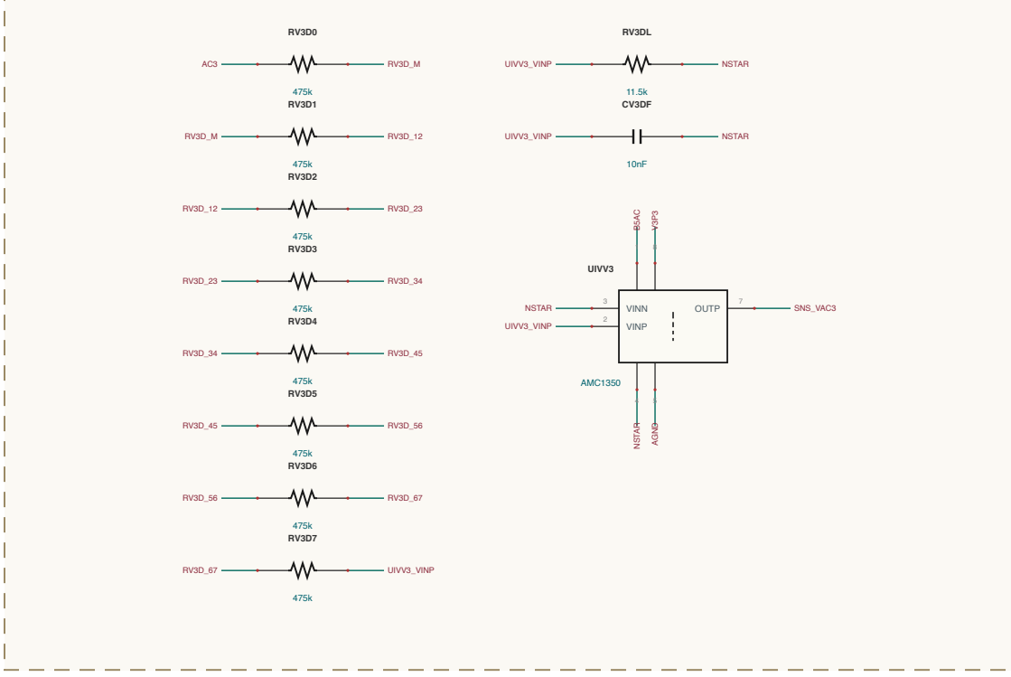
AC-SENSING / SENSE-VAC3
