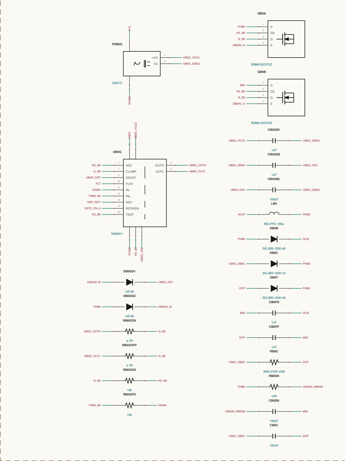
VIENNA-PFC / PHASE-B0
