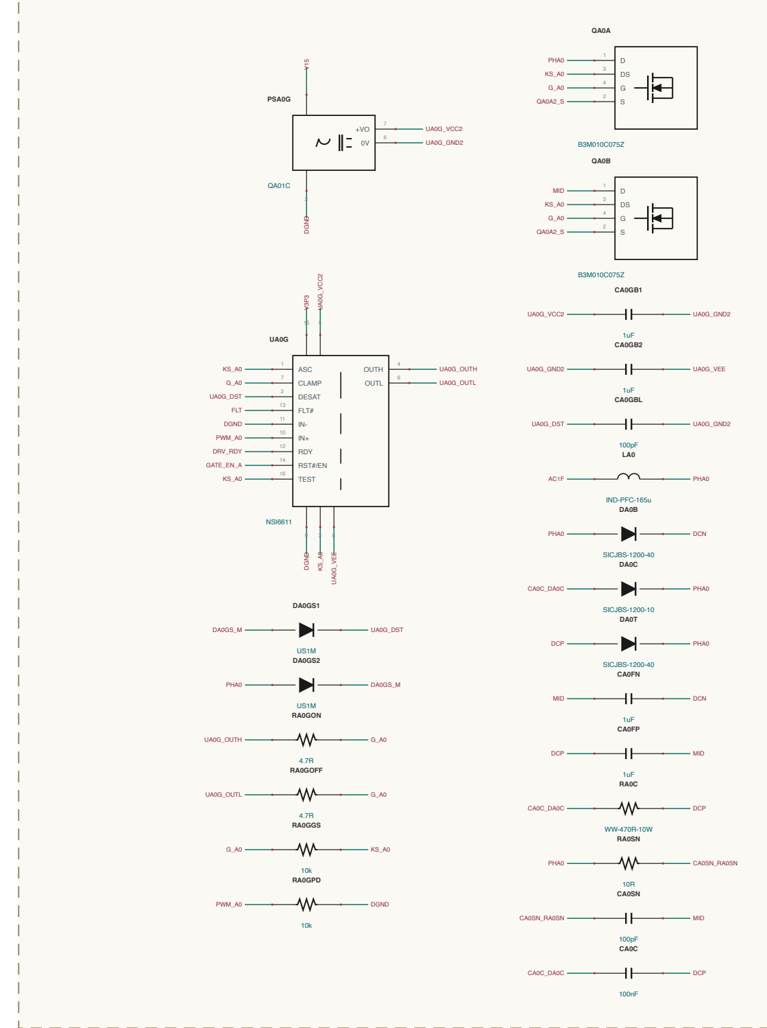
VIENNA-PFC / PHASE-A0
