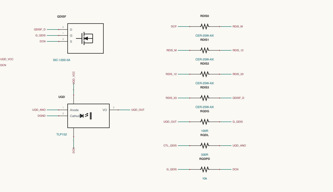
CONTROL / GROUNDING
