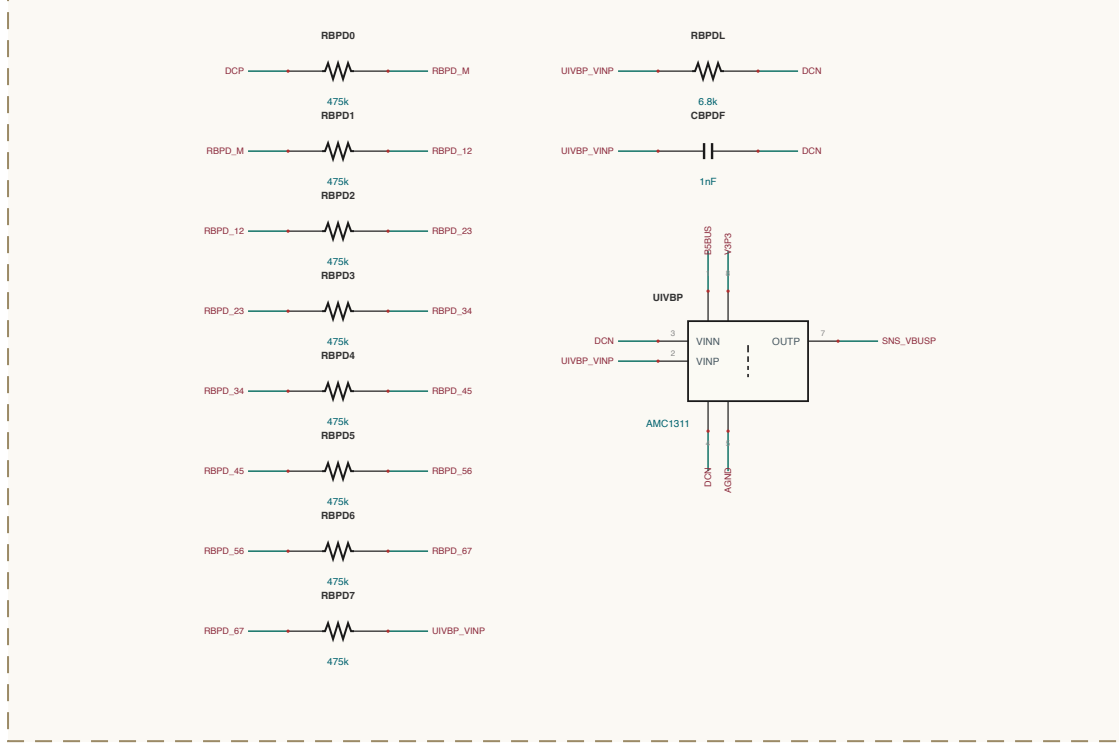
AC-SENSING / SENSE-VBUS
