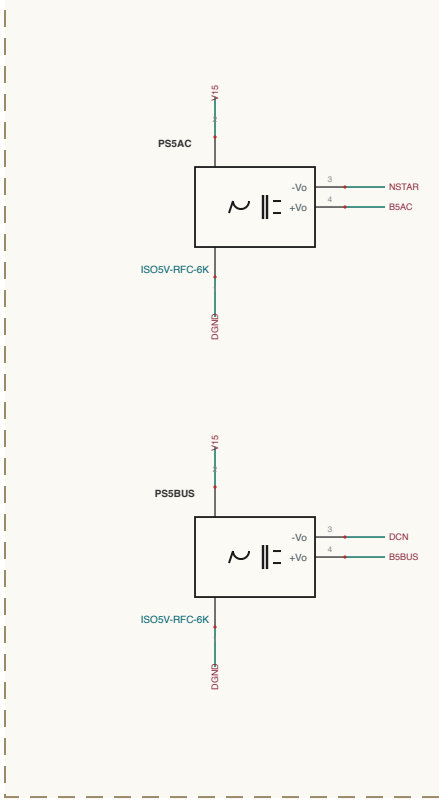
AC-SENSING / ISO-BIAS
