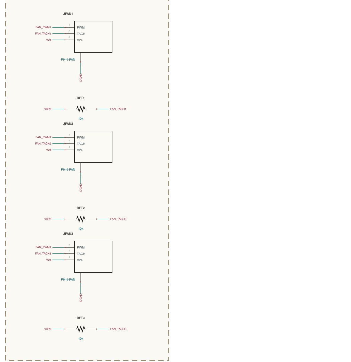
AUX-POWER / FANS
