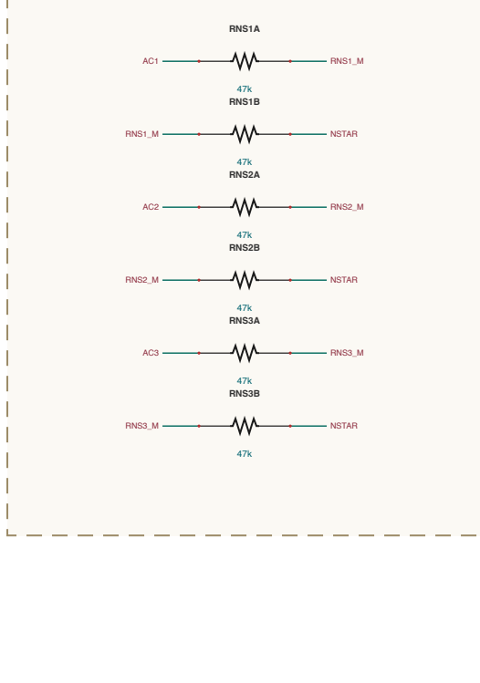
AC-SENSING / STAR
