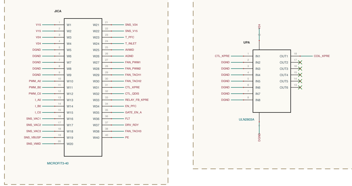
AUX-POWER / INTERCONNECT
