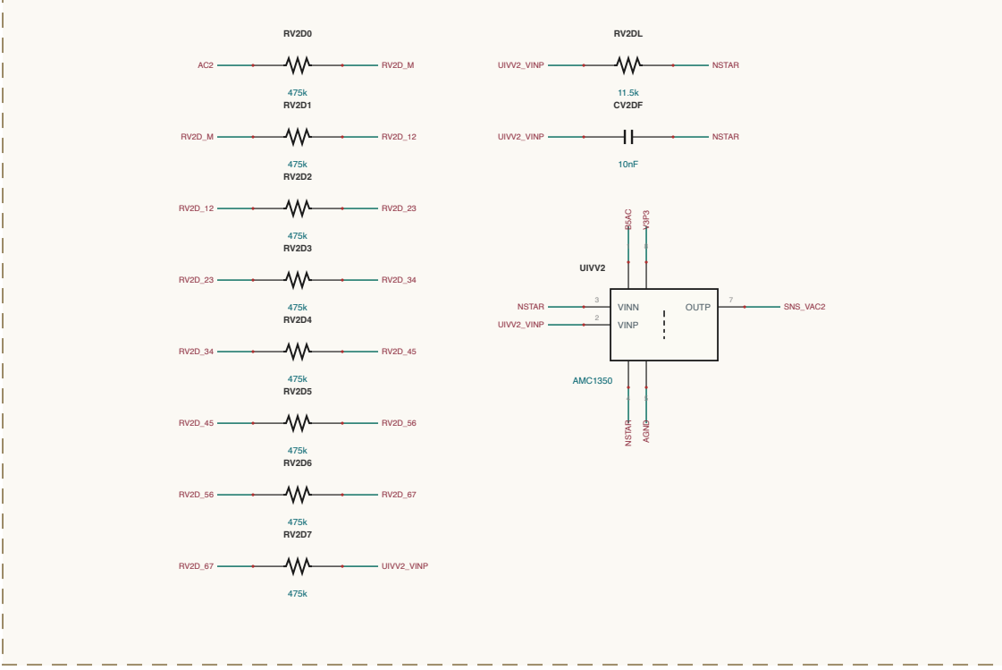
AC-SENSING / SENSE-VAC2
