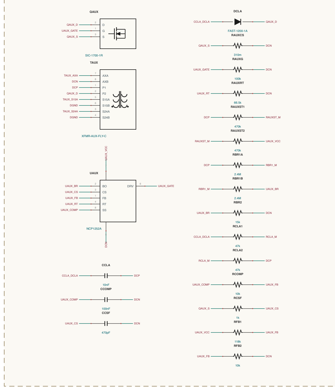
AUX-POWER / FLYBACK
