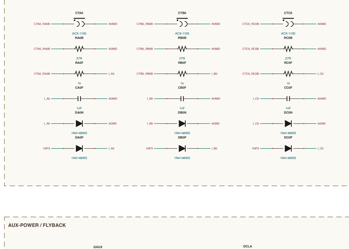
AC-SENSING / LINE-CTS-0
