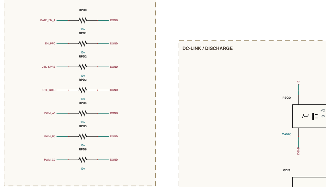
CONTROL / CARD-UP
