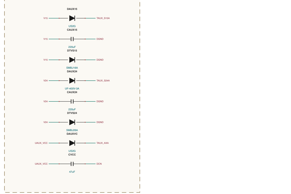
AUX-POWER / RAILS
